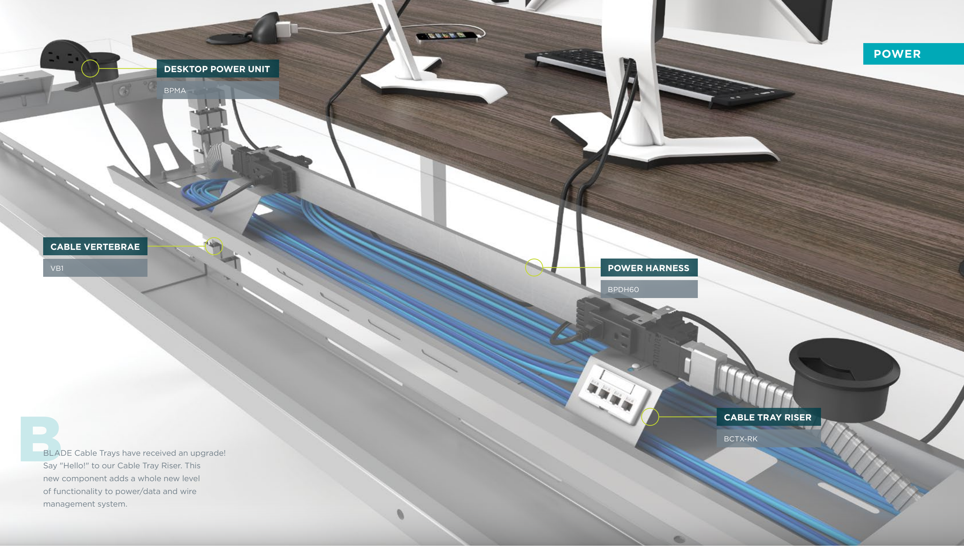
CABLE TRAY RISER: Lifts Harness from Tray, allowing wires to flow underneath. Also houses Data Faceplate.
